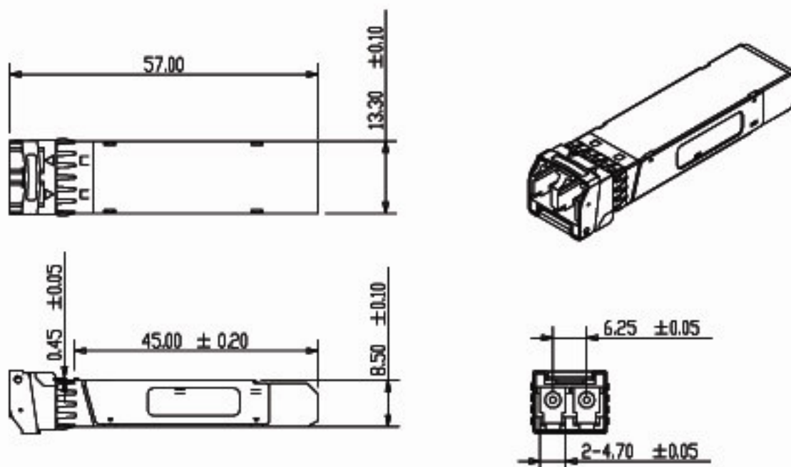
Figure4. Mechanical Specifications
